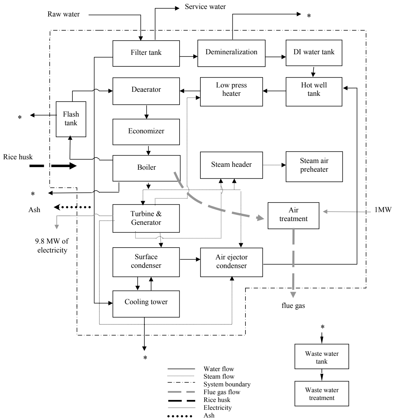
Figure 1. System boundary of rice husk energy production
